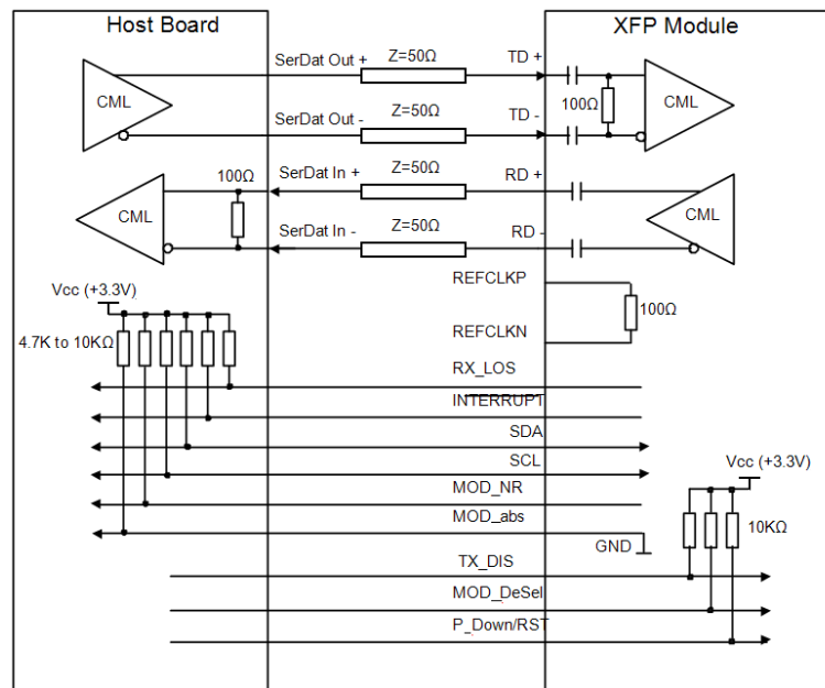
Recommended High-speed Interface Circuit
