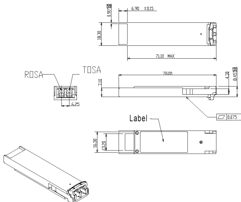
Figure3. Mechanical Specifications
