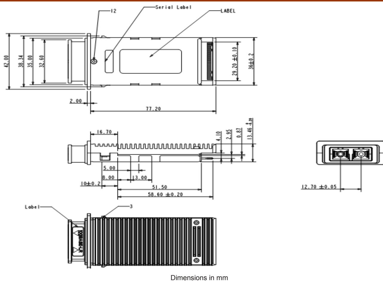
Figure3. Mechanical Dimensions
