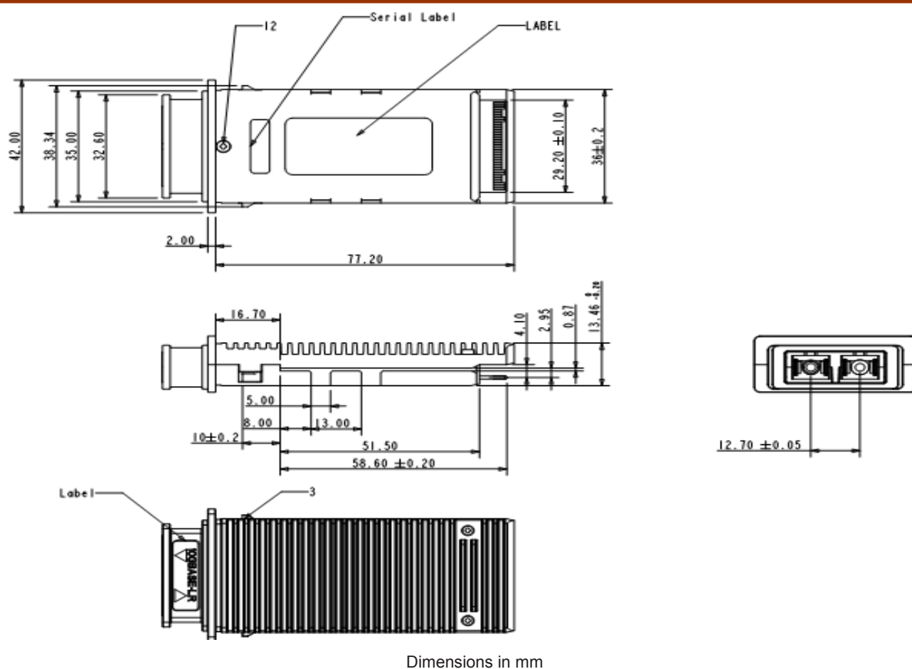
Figure3. Mechanical Dimensions
